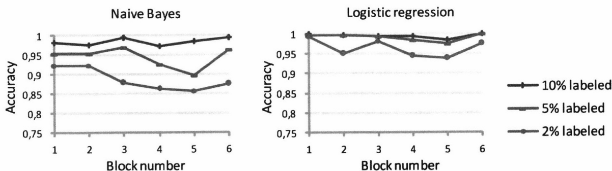
Fig. 2. Classification results of NB and LR for mushroom data set. (Colours are visible in the online version of the article; http://dx.doi.org/10.3233/IDA-2011-0488 )
